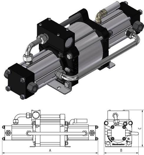
DLE 5 double acting, single air drive head single stage
