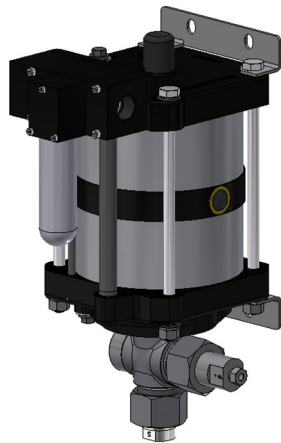
G100-2 (L) single acting, double air drive head (Standard= Bottom inlet)
