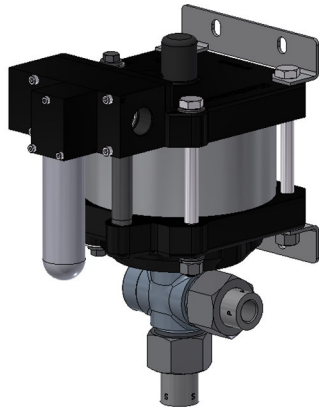
G100 (L) single acting, single air drive head (Standard= Bottom inlet)
