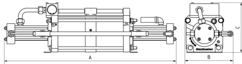
DLE 15-75-2 single acting, double air drive head two stages
