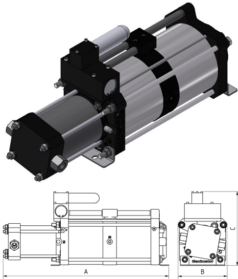
DLE 2-1-2 single acting, single air drive head single stage
