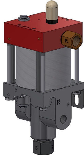
MO72 Single acting, single air drive head (Standard= Bottom inlet)
