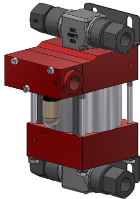
M189D double acting, single air drive head (Standard= Side inlet)
