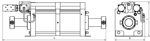
GPD180-2 double acting, double air drive head
