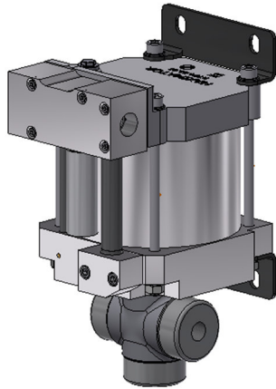
S40-SS single acting, single air drive head
