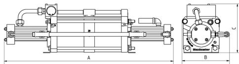
DLE 30-75-2 double acting, double air drive head two stages
