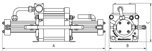
DLE 15-75 single acting, single air drive head two stages
