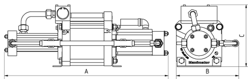
DLE 5-15 single acting, single air drive head two stages
