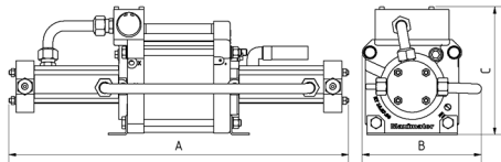
DLE 30 double acting, single air drive head single stage
