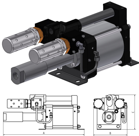
GX60 double acting, single air drive head (Standard= Bottom inlet)
