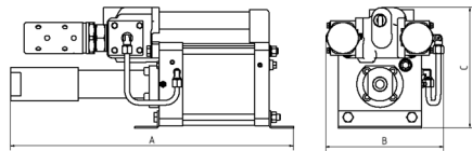
GX100 double acting, single air drive head (Standard= Bottom inlet)
