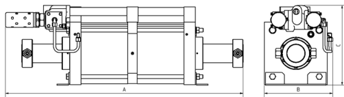
GPD120-2 double acting, double air drive head
