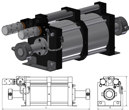
GPD180-2 double acting, double air drive head
