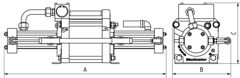
DLE 30-75 single acting, single air drive head two stages
