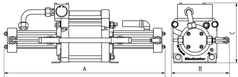
DLE 15-30 single acting, single air drive head two stages
